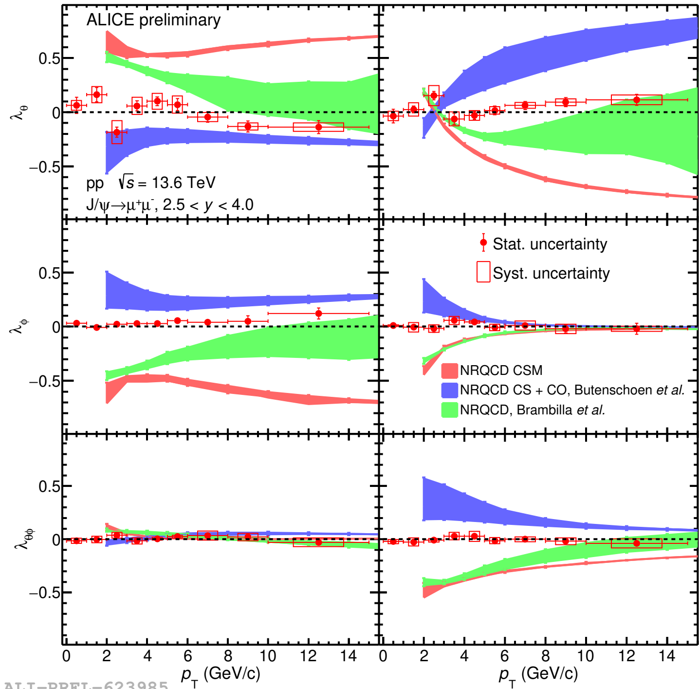
Collins-Soper
