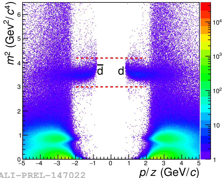
deuteron m^2 vs momentum (tracks crossing TRD) data
