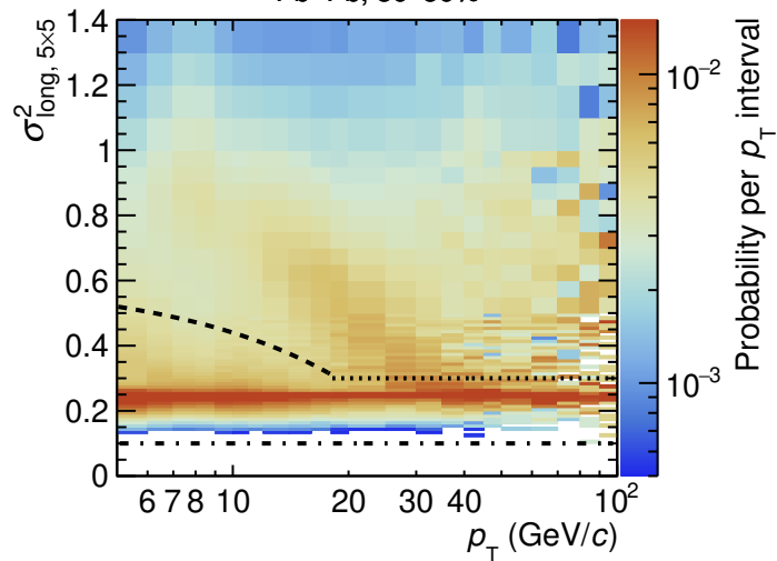
Pb-Pb, 30-50%
